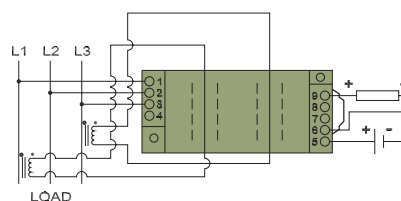
CR6240 CR6241 3 element - 3 Wire, 4 - 20 mADC Output with external current transformer
