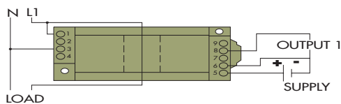
CR6210 CR6211 Single element, 0 - 5 VDC Output
