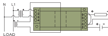
CR6220 CR6221 Single element, 4 - 20 mADC Output with external voltage transformers
