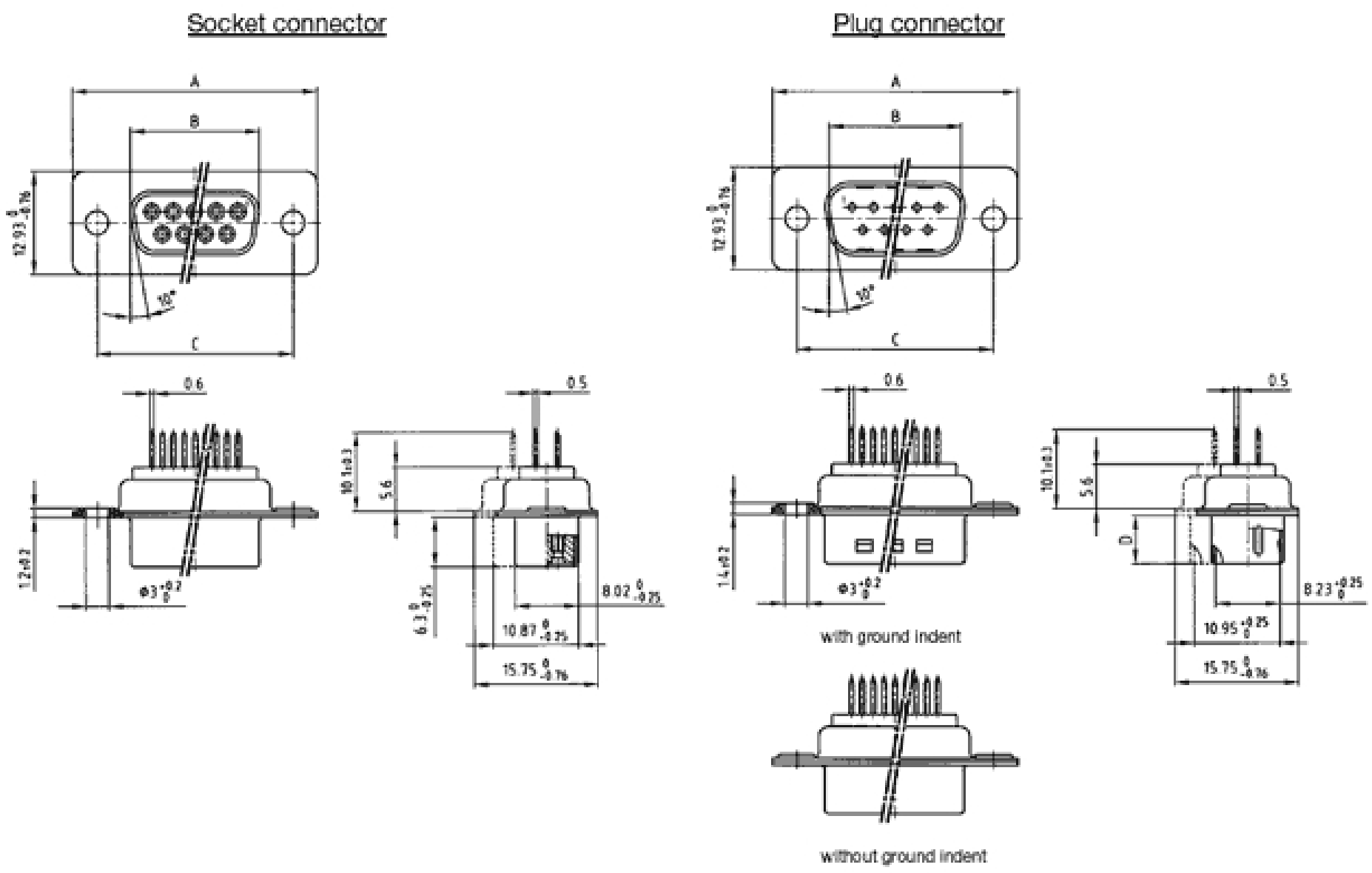
Socket connector:
