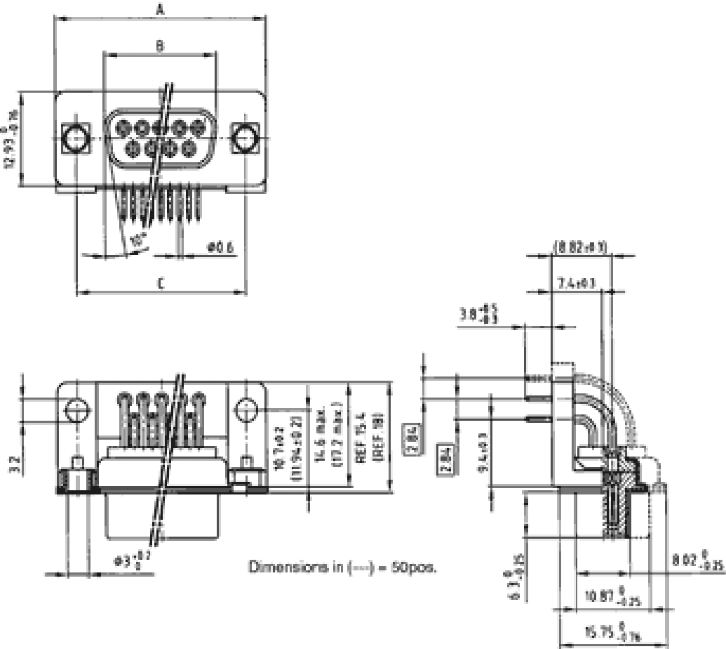
Socket connector
