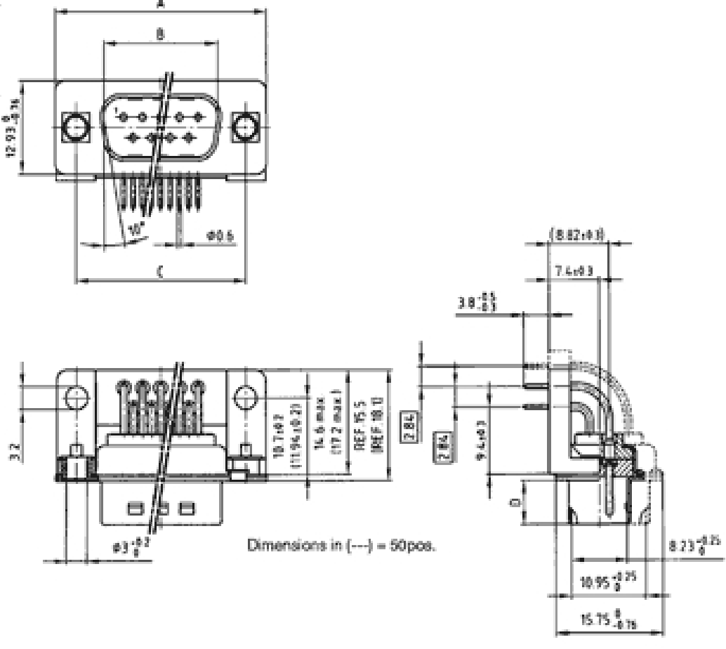
Plug connector
