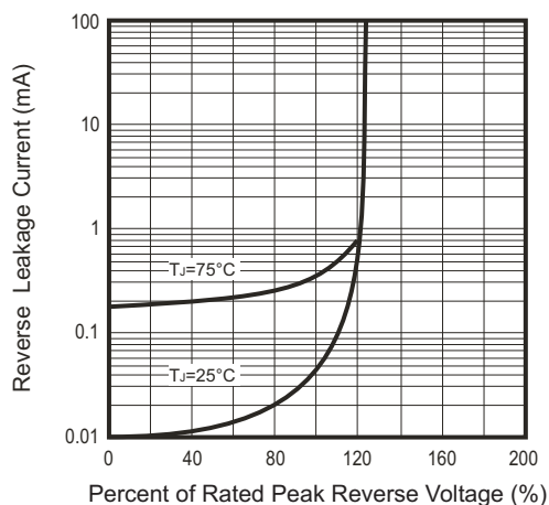
Fig.5- Reverse Characteristics
