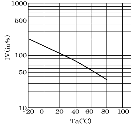
IV-Ta Characteristics
