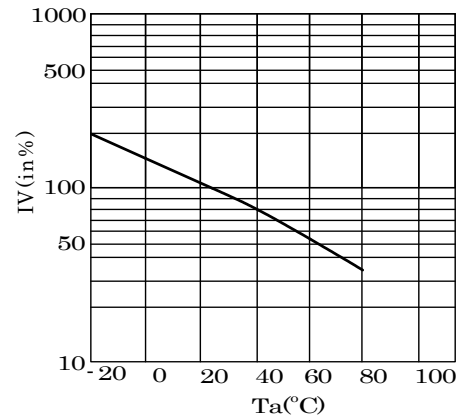
IV-Ta Characteristics
