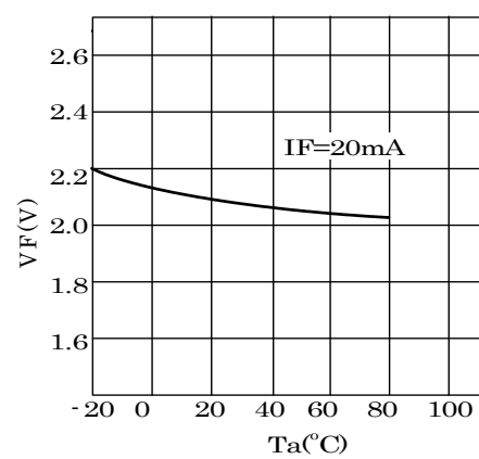
VF-Ta Characteristics
