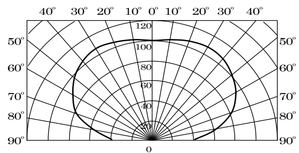
Directive Characteristics
