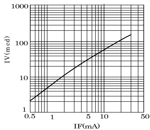
IV-IF Characteristics
