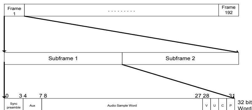
Figure 33 S/PDIF Format
