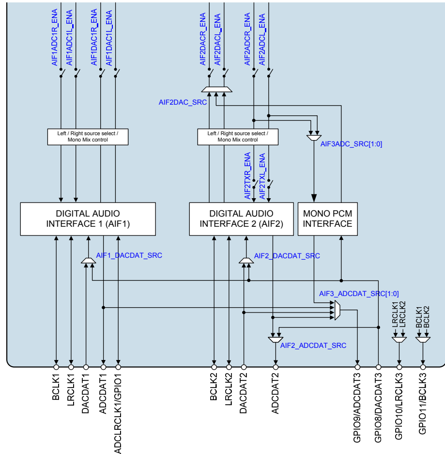
Figure 66 Audio Interface AIF3 Configuration
