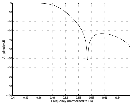
Figure 29. ADC Transition Band
