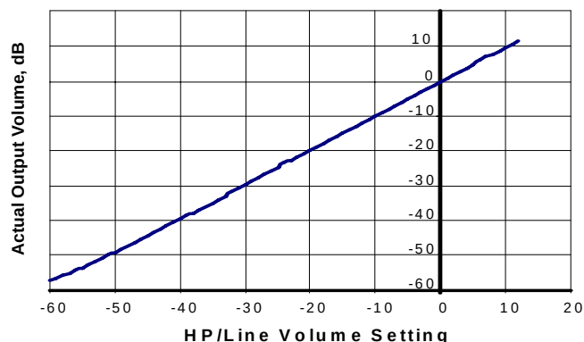
Figure 26. HP/Line Output Volume vs. Volume Setting
