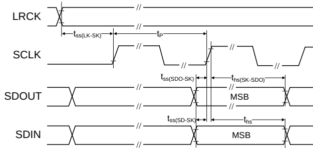
Figure 5. Serial Port Timing (Slave Mode)
