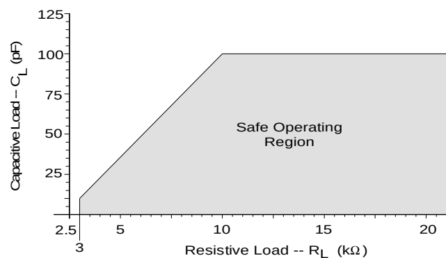
Figure 3. Maximum Loading
