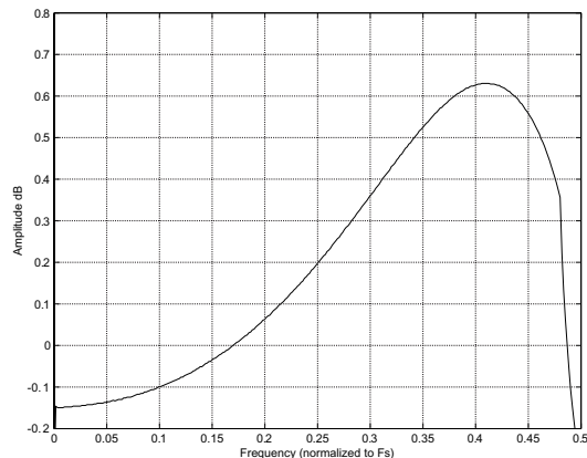
Figure 31. DAC Double-Speed Passband Ripple
