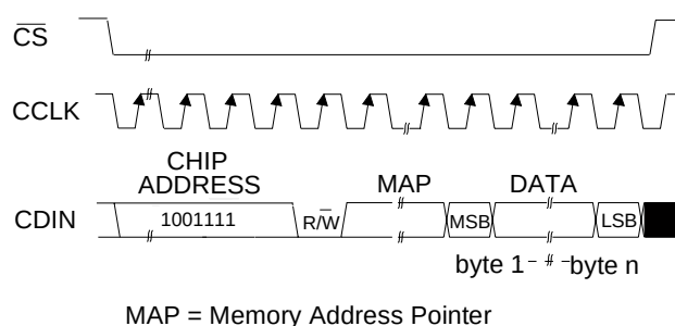
Figure 21. Control Port Timing, SPI Mode
