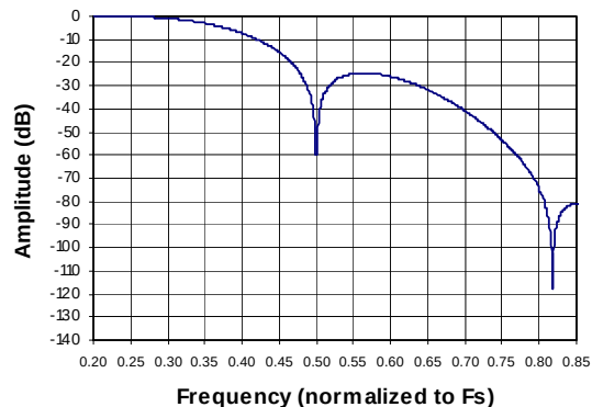
Figure 45. ADC Quad-Speed Stopband (detail)
