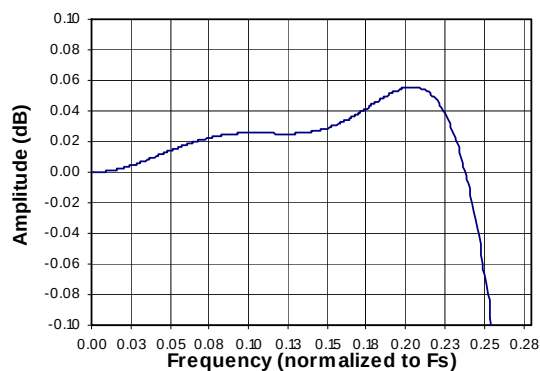
Figure 47. ADC Quad-Speed Passband Ripple
