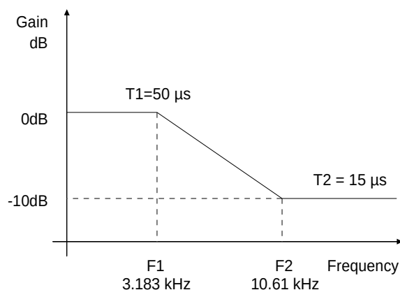
Figure 23. De-Emphasis Curve
