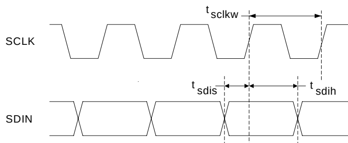
Figure 8. Master and Slave Mode SDIN vs. SCLK
