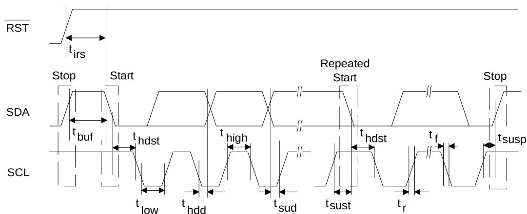
Figure 12. I 2 C Mode Control Port Timing
