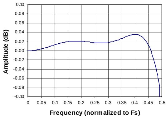
Figure 39. ADC Single-Speed Passband Ripple
