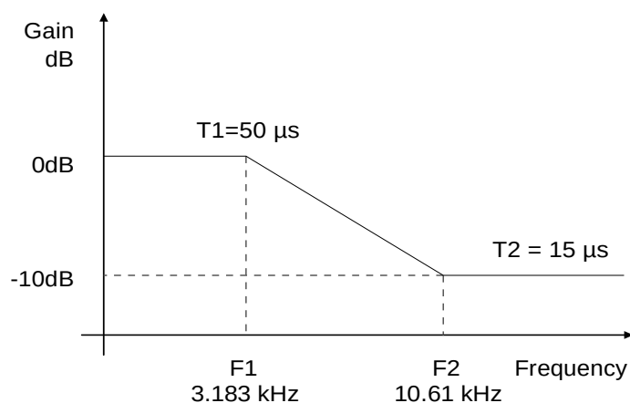
Figure 14. De-Emphasis Curve
