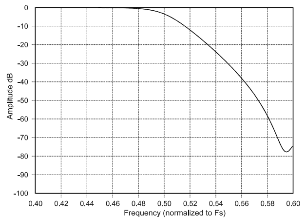
Figure 29. DAC Double-Speed Transition Band
