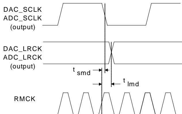
Figure 1. Serial Audio Port Master Mode Timing
