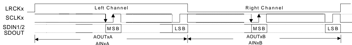
Figure 15. Right-Justified 16-Bit Data, Right-Justified 24-Bit Data
