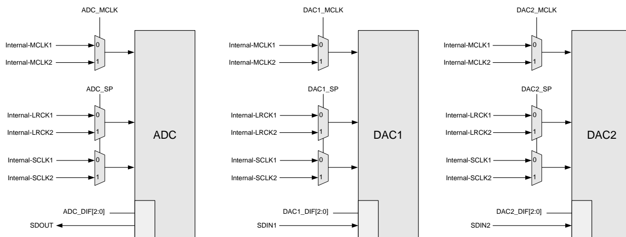
Figure 11. Converter Clocking
