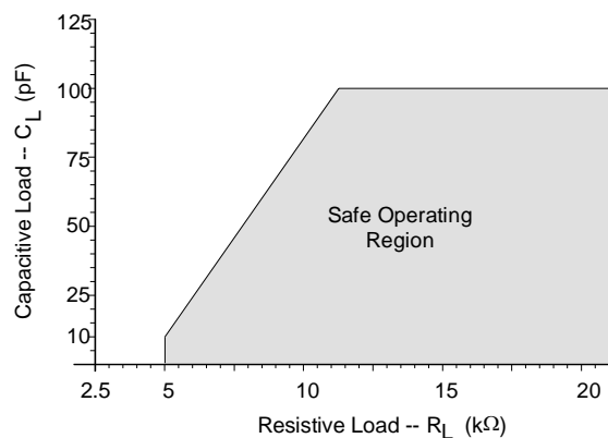
Figure 2. Maximum Analog Line Output Loading
