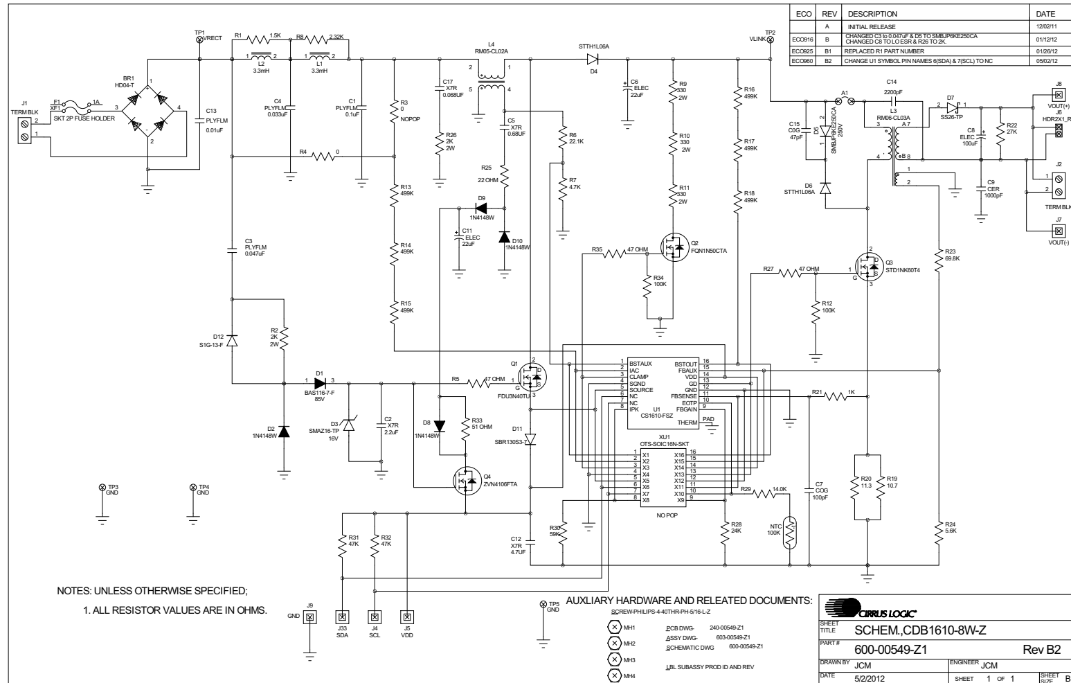
Figure 1. Schematic
