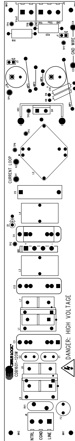
Figure 5. Silkscreen (Top)
