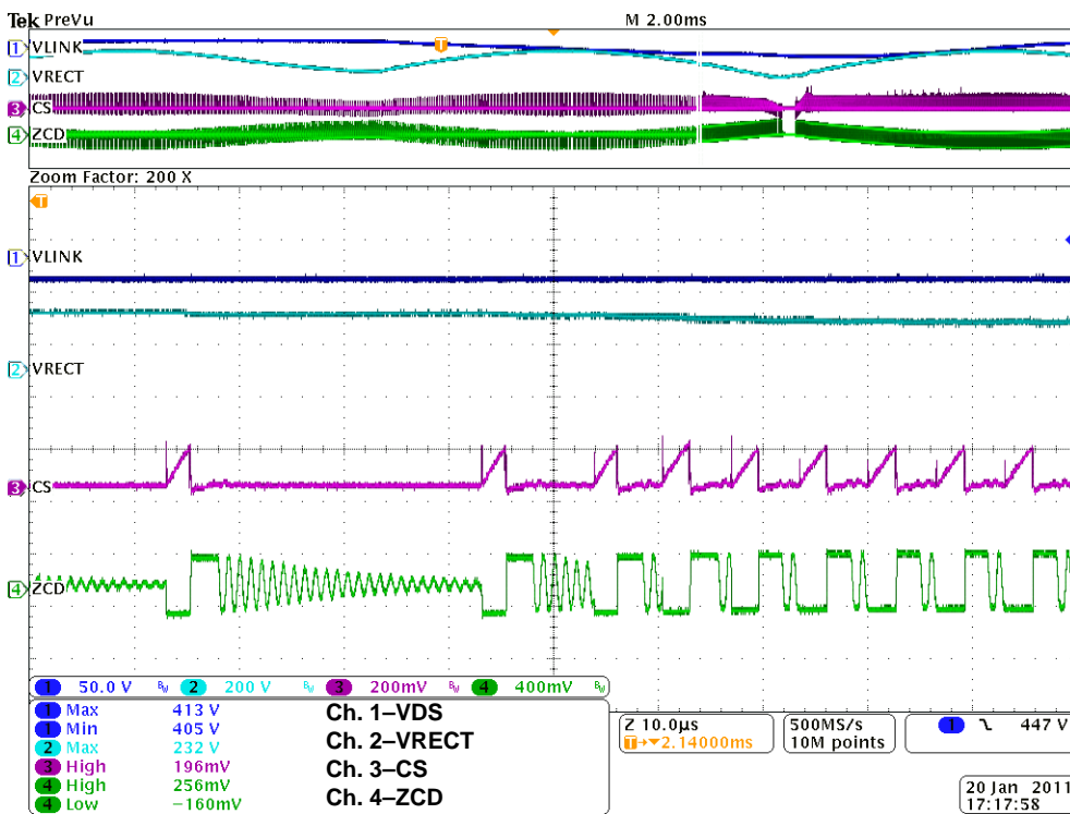
Figure 33. Transient — 15W to 115W Load at 10W/μs, Vin = 277VAC (cont.)
