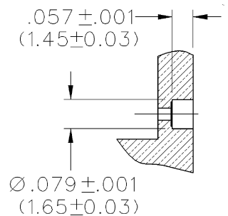
Mounting Hole Layout
