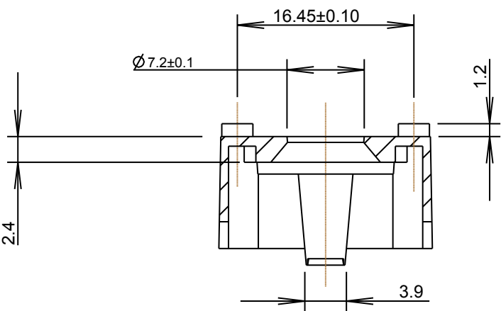
SECTION X-X
