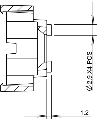
SECTION Y-Y
