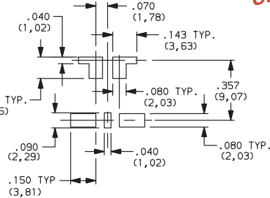
ET01J6SAKE2 Horizontal Actuation SPDT
