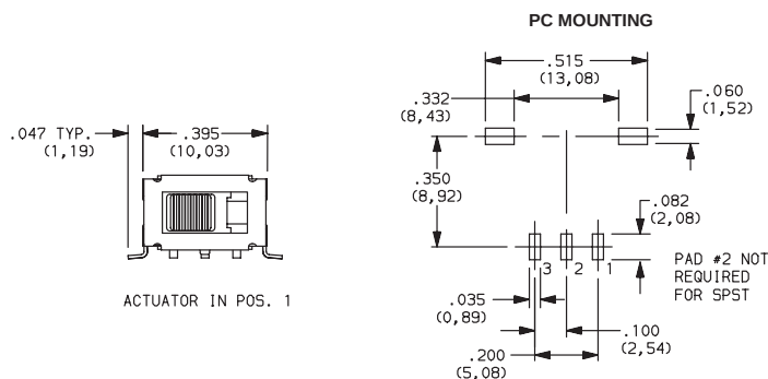
ES01MSAKE Horizontal Actuation SPDT
