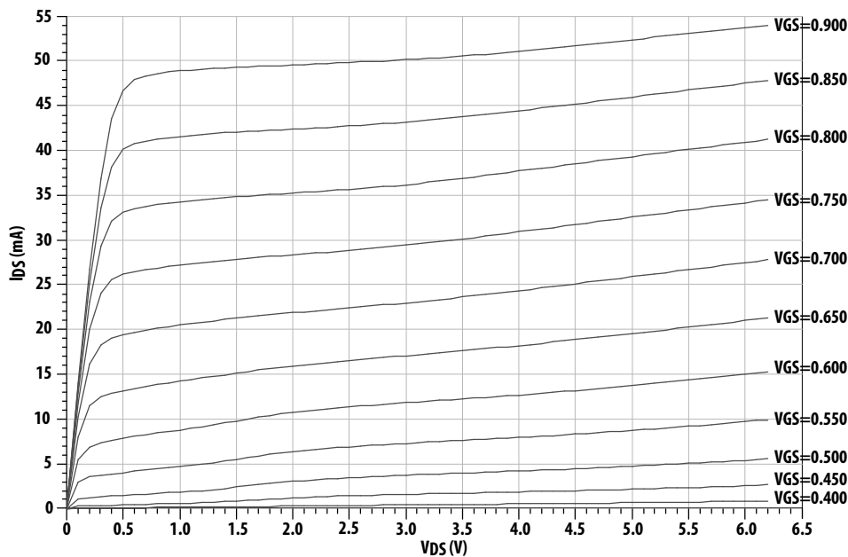
Figure 1. Typical I-V Curves. ( V_{GS}=0.05\text{ V} per step)
