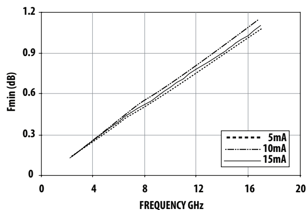
Figure 10. NFmin vs. Frequency at 2V
