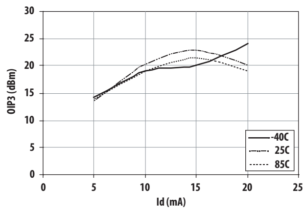
Figure 14. OIP3 vs. Ids at 12 GHz over temp at 3V
