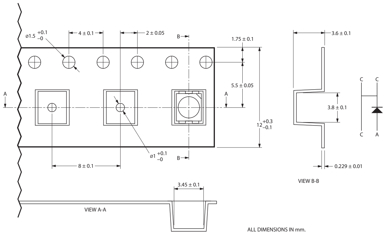
Figure 13. Tape dimensions
