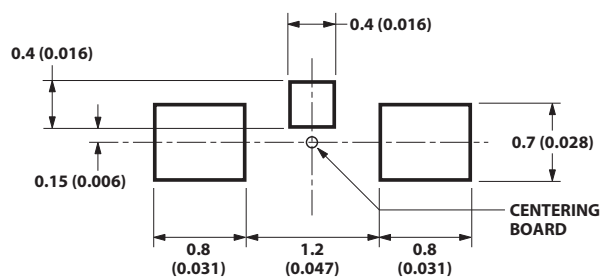
Figure 12. Recommended soldering pad pattern for HSMW-C120.
