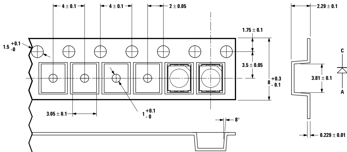
Figure 11. Tape dimension
