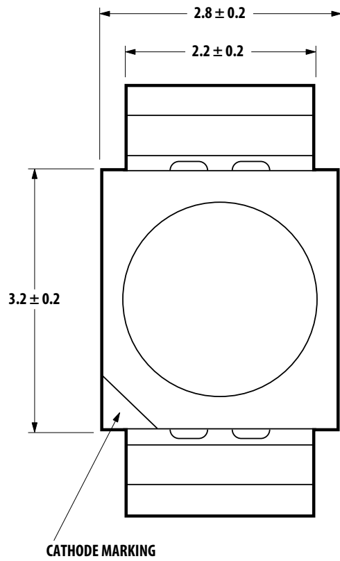
REVERSE MOUNT
