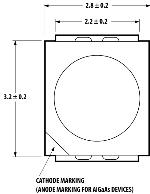
TOP MOUNT
