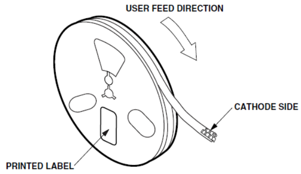
Figure 8. Reel orientation
