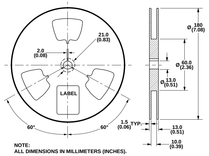
Figure 11. Reel Dimensions.
