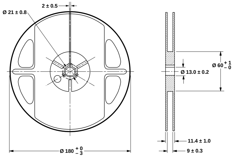
Figure 9. Reel Dimensions.
