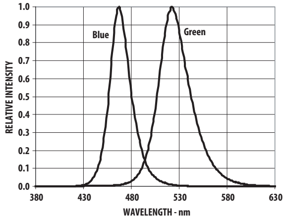
Figure 5. Relative Intensity vs Wavelength
