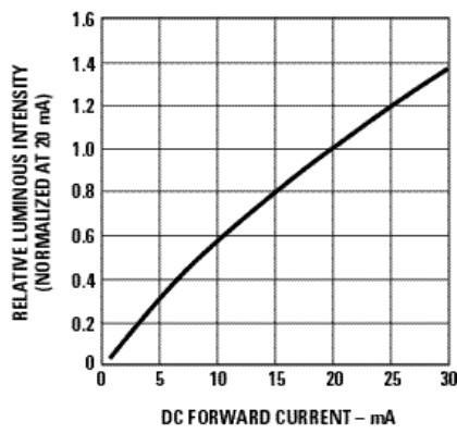
Figure 8. Relative intensity vs. forward current.
