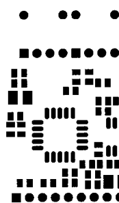
Figure 10c. Top Side Solder Mask
