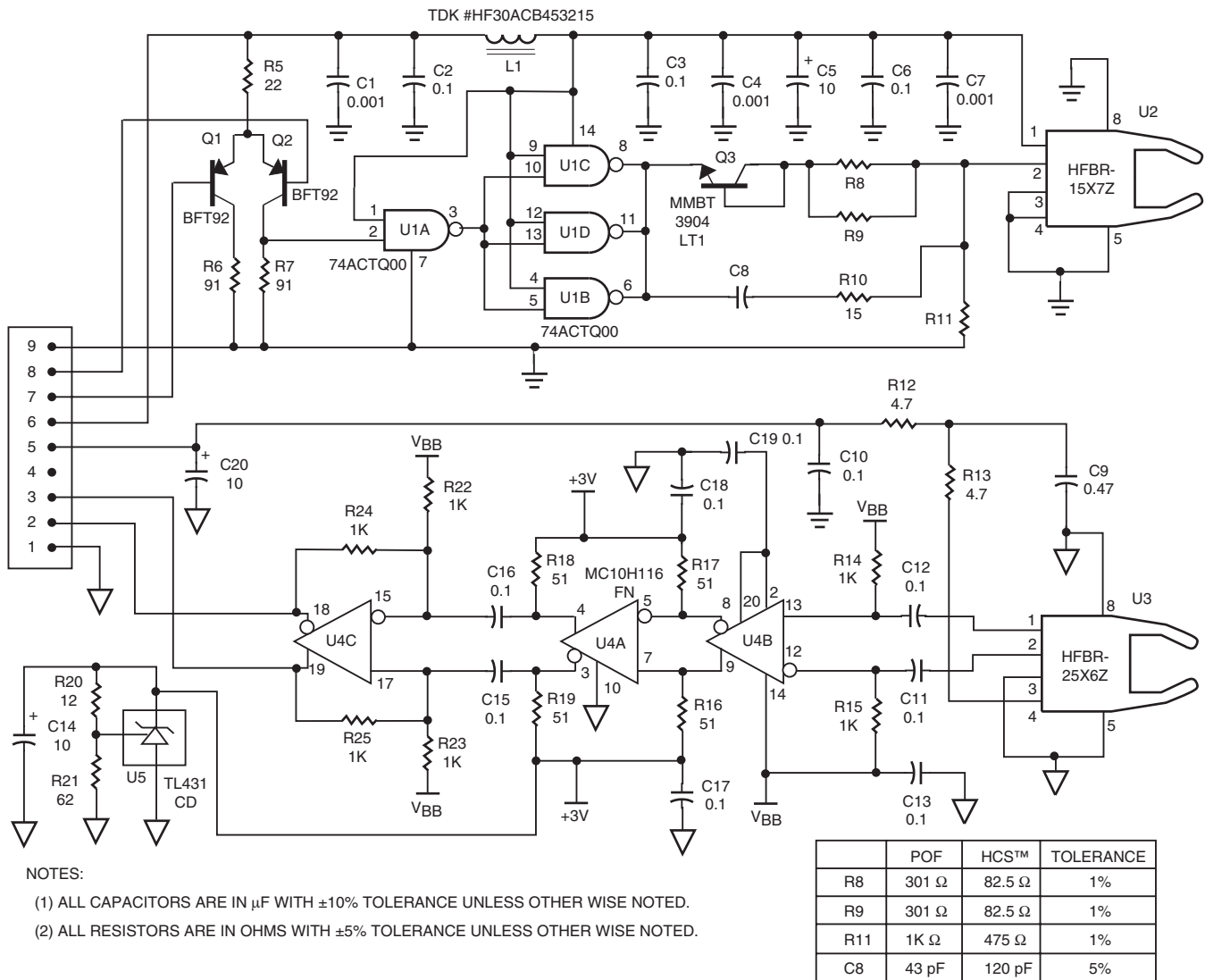
Figure 8. Fiber Optic Transceiver Using Surface Mount Components
