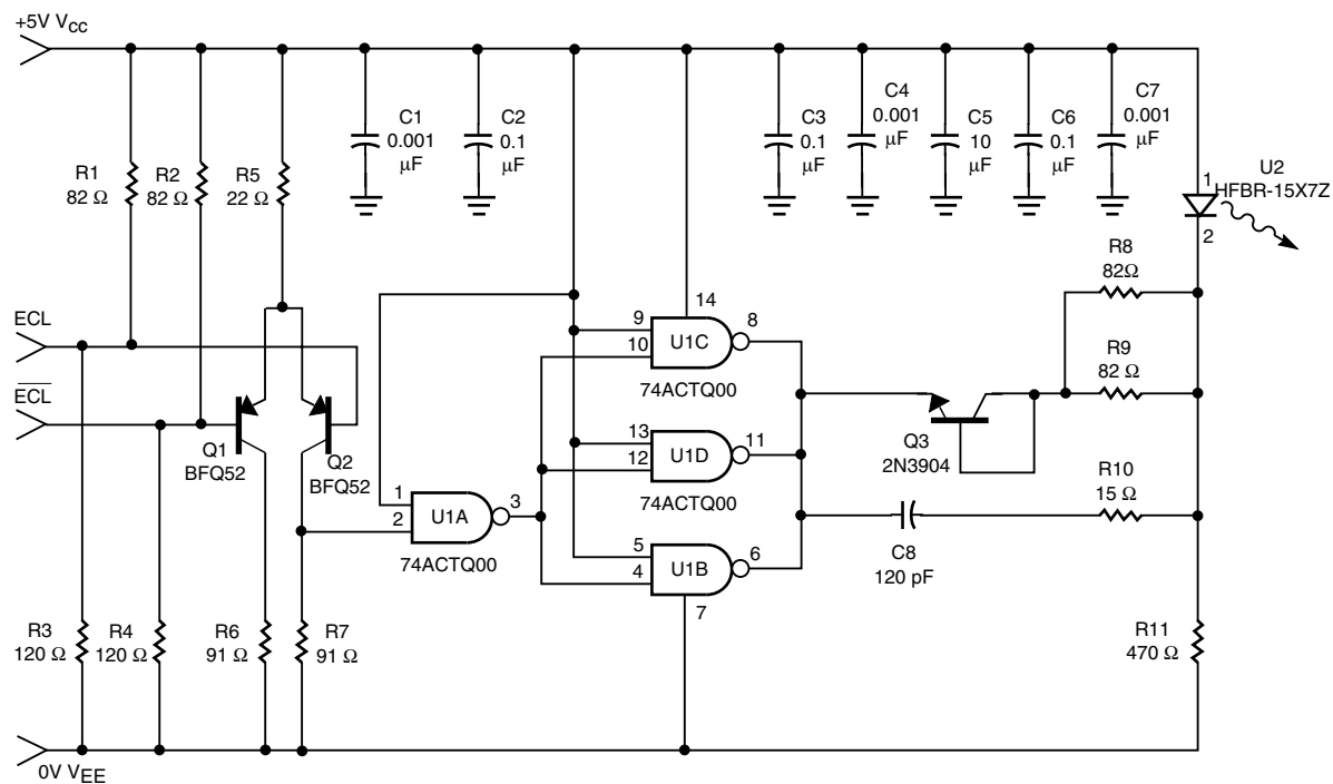
Figure 6. +5 V ECL Through Hole Transmitter for 200 \mu\text{m} HCST TM Fiber
