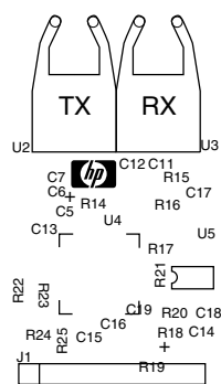
Figure 10b. Top Silkscreen
