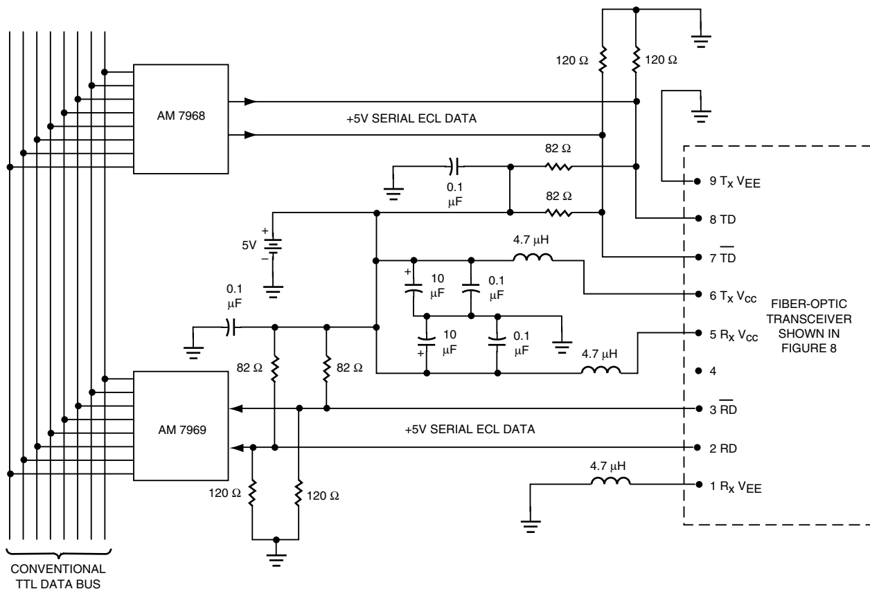
Figure 11. Byte-to-Light Transceiver
