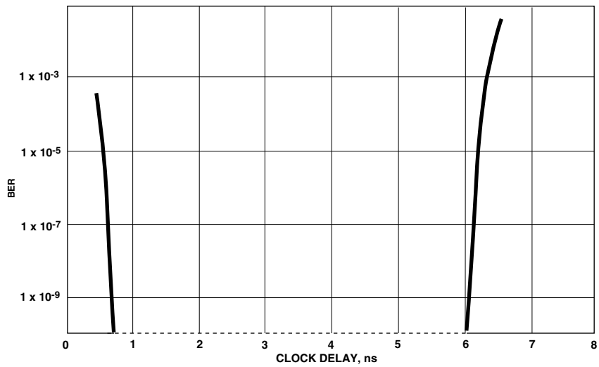
Figure 16. Typical BER vs. Clock Delay at 125 MBd with 100 m of 200 \mu m HCS™ Fiber
