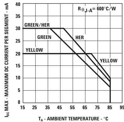
Figure 9. Maximum Allowable DC Current vs. Ambient Temperature. T_{\text{JMAX}} = 100^{\circ}\text{C} .
