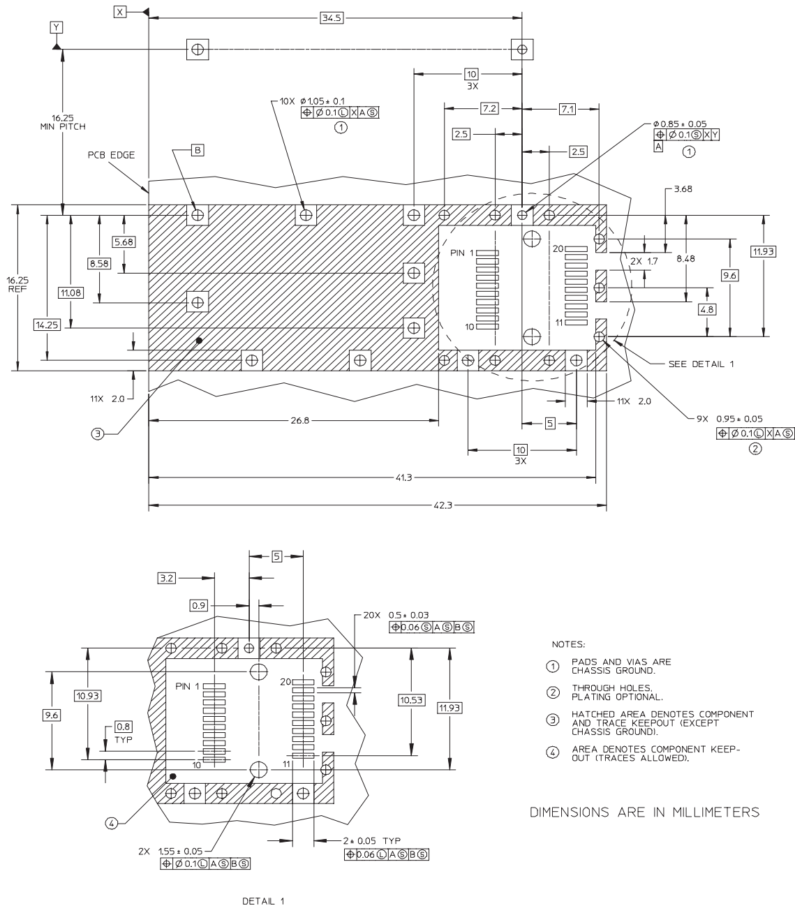
Figure 7d. SFP Host Board Mechanical Layout
