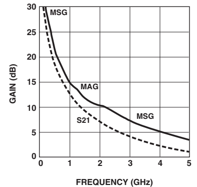
Figure 17. AT-41533 Gains vs. Frequency at V_{CE} = 5V , I_C = 25 \text{ mA} .
