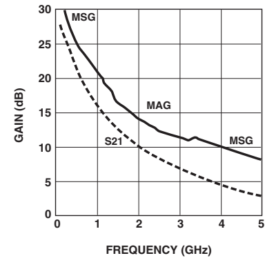
Figure 18. AT-41511 Gains vs. Frequency at V_{CE} = 8V , I_C = 10 \text{ mA} .
