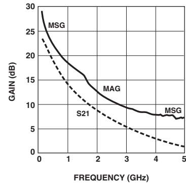
Figure 10. AT-41511 Gains vs. Frequency at V_{CE} = 2.7 \text{ V} , I_C = 5 \text{ mA} .
