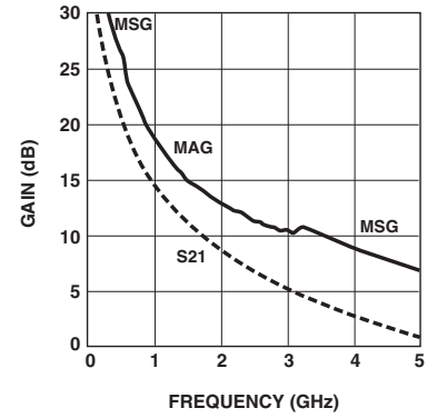
Figure 16. AT-41511 Gains vs. Frequency at V_{CE} = 5V , I_C = 25 \text{ mA} .
