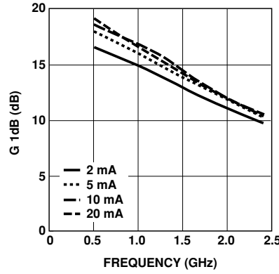
Figure 6. AT-32011 1 dB Compressed Gain vs. Frequency and Current at V_{CE} = 2.7\text{ V} .
