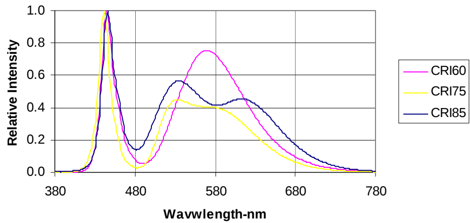
Spectrum Distribution
