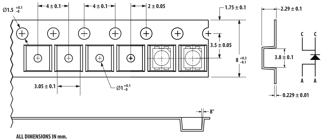
Figure 16. Tape Dimensions
