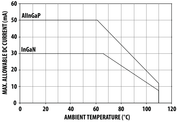
Figure 5a. Maximum forward current vs. ambient temperature. Derated based on T_{jMAX} = 125^{\circ}C . (3 chips)
