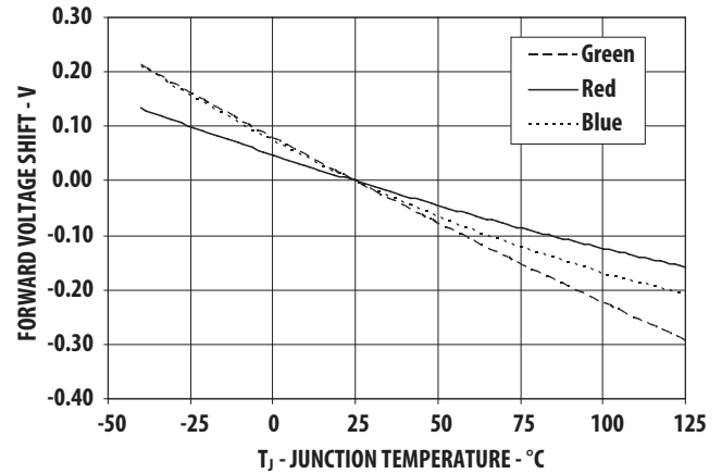
Figure 9. Forward Voltage Shift vs Junction Temperature
