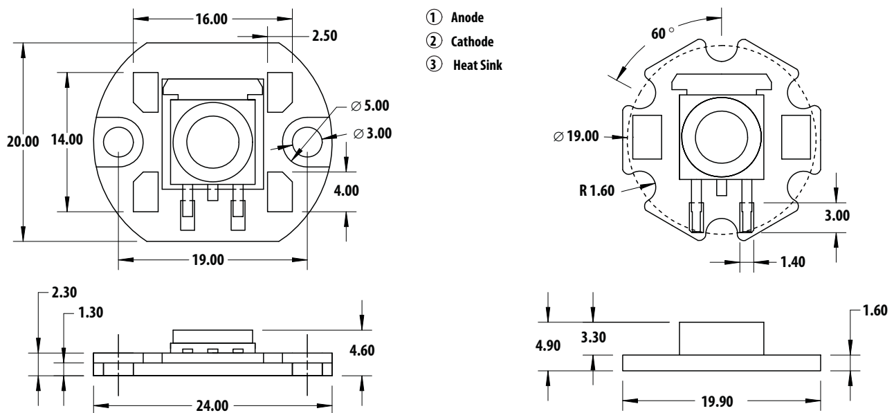
Figure 2. MCPCB I package outline drawing.
