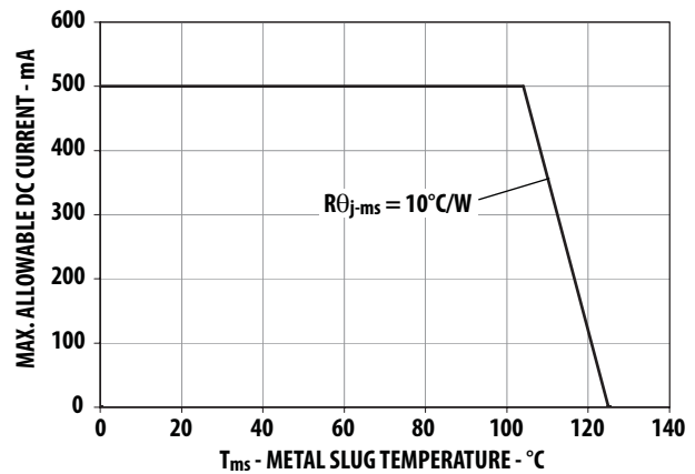
Figure 13. Maximum forward current vs. metal slug temperature
