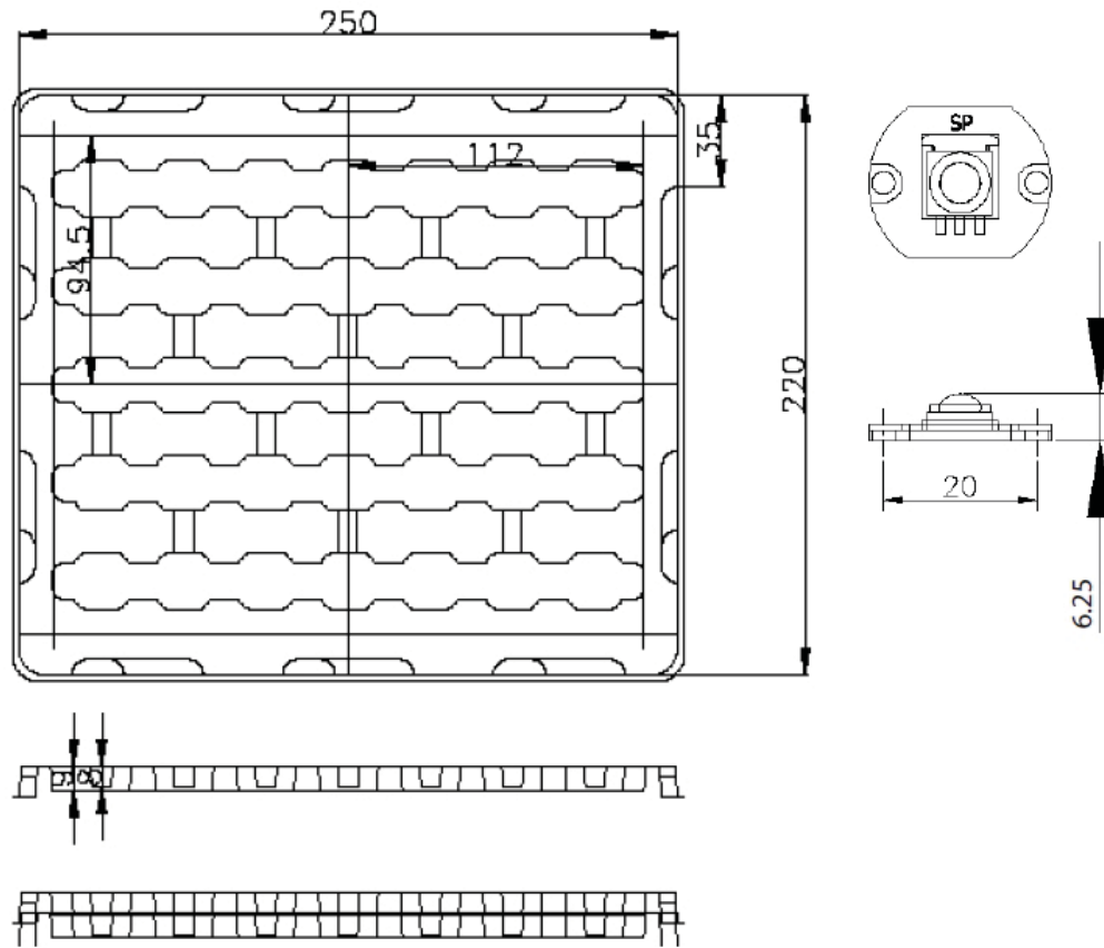
Figure 22. Tray dimensions.
