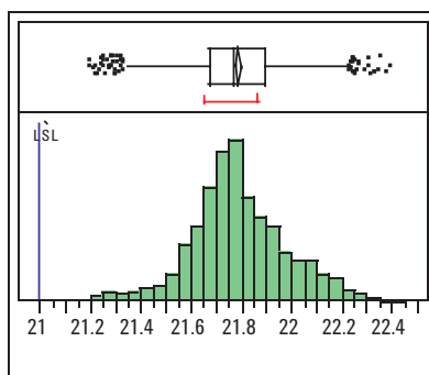
Noise Figure at 26 GHz
