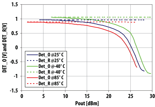
Figure 15. Detector voltages vs. Output Power at Freq = 42 GHz
