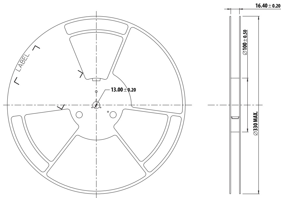
Figure 11. Reel Dimension
