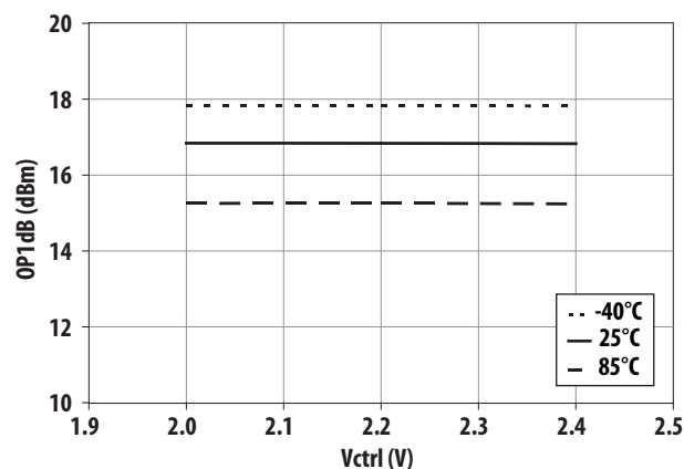
Figure 21. OP1dB vs Vctrl and temperature
