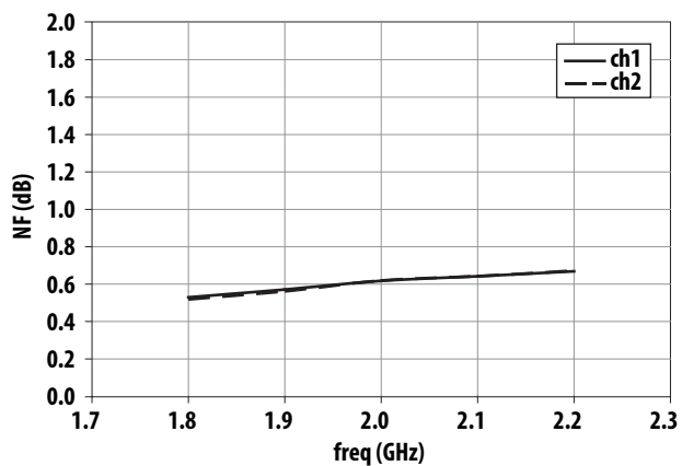
Figure 9. NF vs Frequency and channel
