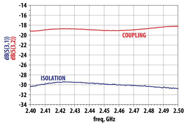
Figure 10. TX Coupling Coefficient and Coupler Isolation vs Frequency
