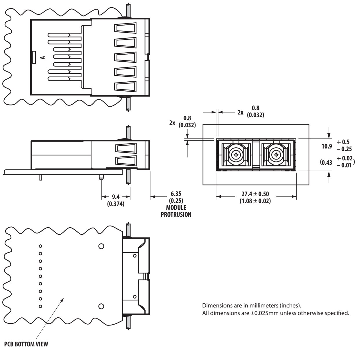
Figure 8b. Dimensions shown for mounting module with extended shield to panel.
