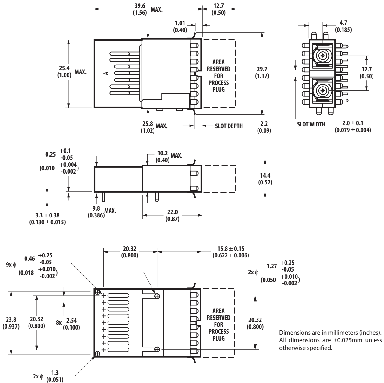
Figure 2c. Package outline drawing with mezzanine height and flush shield.
