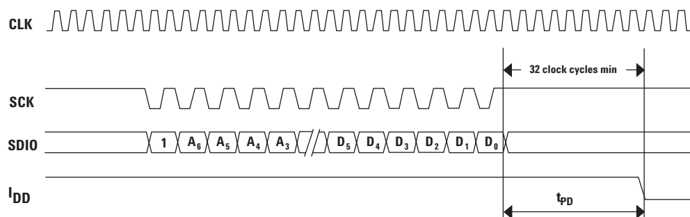
Figure 12. Power-down timing.
