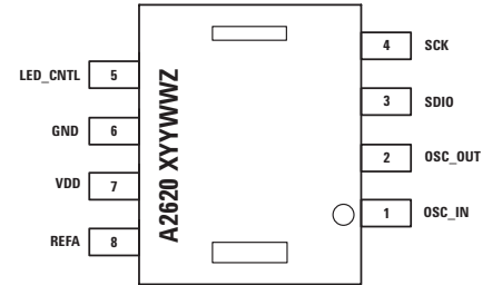
Figure 1. Mechanical drawing: top view.
