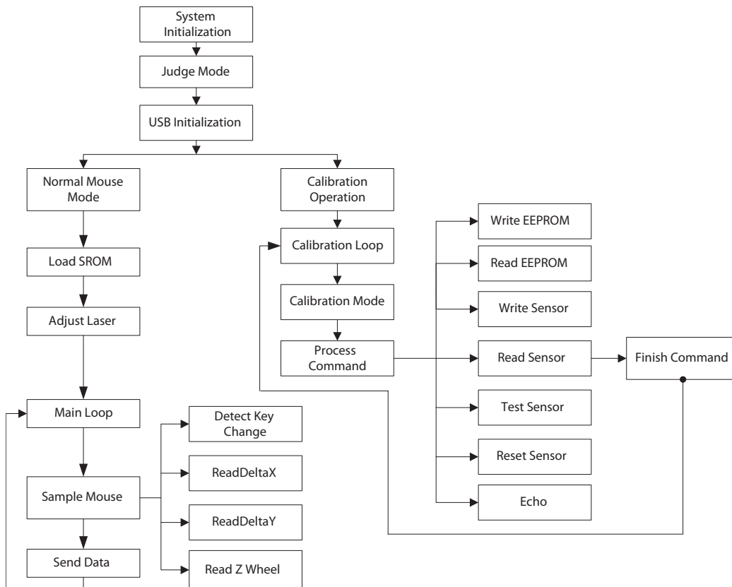
Figure 6. USB Operation Function Call Map
