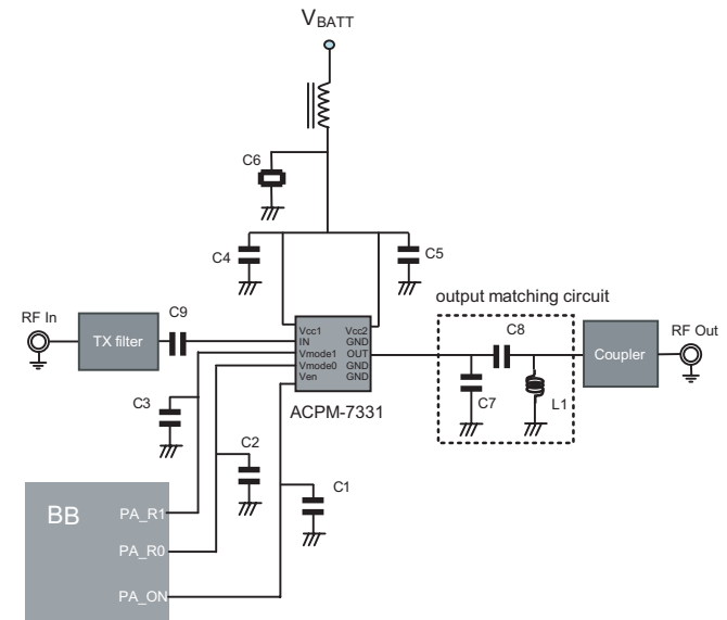
Figure 16. Peripheral Circuits
