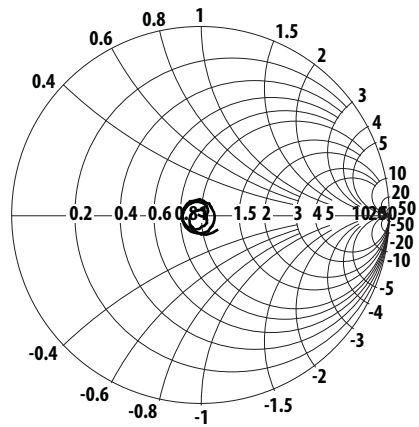
Figure 16. Ant Port Impedance in Rx Band
