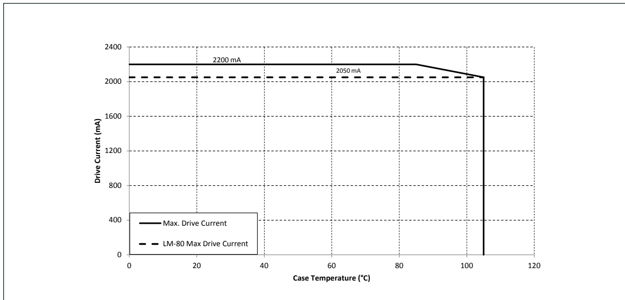
Figure 1: H12 Drive Current Derating Curve (T j = T c = 25°C)
