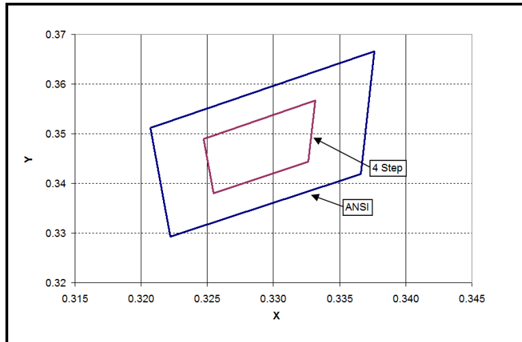
Figure 15: Graph of 5600K Cool White Test Bins in xy Color Space
