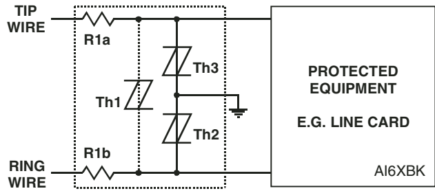
Figure 17. Protection Module
