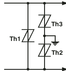
Figure 12. Multi-point Protection
