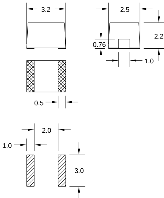
Pad Layout
